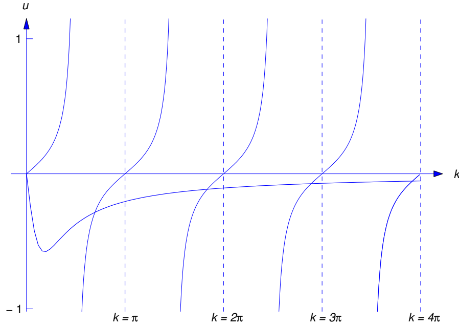
Figure 13.2.2 u = \tan k and u = -2k/(1 + 3k^2)
