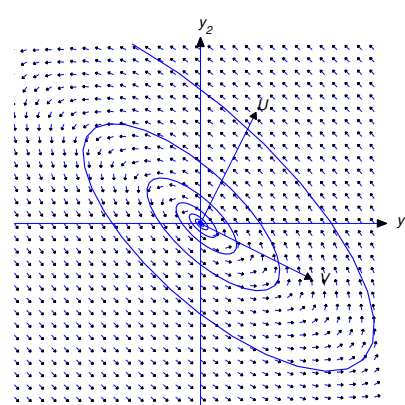
Figure 10.6.4 \alpha > 0 ; trajectory spiraling outward
