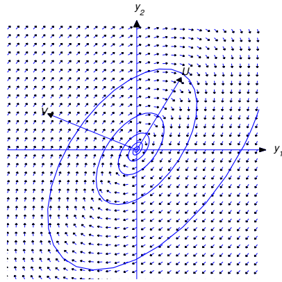
Figure 10.6.5 \alpha < 0 ; trajectory spiraling inward Figure 10.6.6 \alpha < 0 ; trajectory spiraling inward
