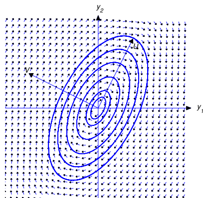
Figure 10.6.1 Shadow trajectories traversed clockwise
