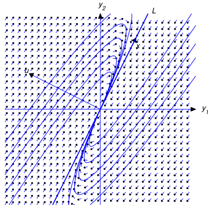
Figure 10.5.4 Negative eigenvalue; motion toward the origin
