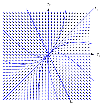
Figure 10.4.5 Two negative eigenvalues; motion toward the origin
