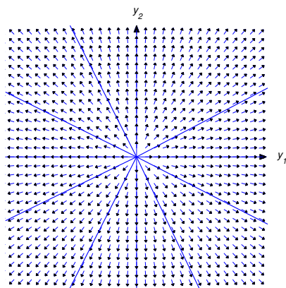
Figure 10.4.1 Trajectories of a 2 \times 2 system with a repeated positive eigenvalue
