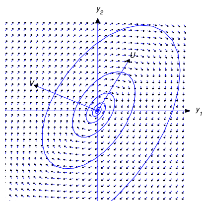
Figure 10.6.3 \alpha > 0 ; trajectory spiraling outward
