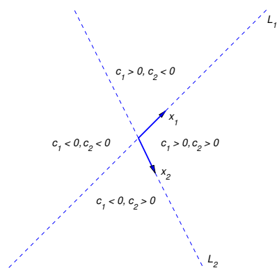
Figure 10.4.3 Four open sectors bounded by L_1 and L_2
