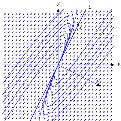
Figure 10.5.2 Positive eigenvalue; motion away from the origin
