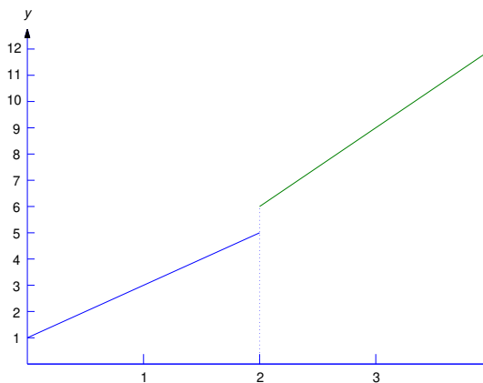
Figure 8.4.1 The piecewise continuous function (8.4.1)
