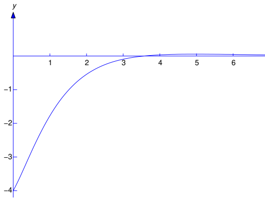
Figure 8.3.1 y = \frac{4}{3}e^{-t/2} - 8e^{-t} + \frac{8}{3}e^{-2t}
