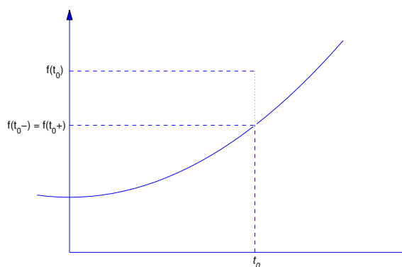
Figure 8.1.2 A removable discontinuity
