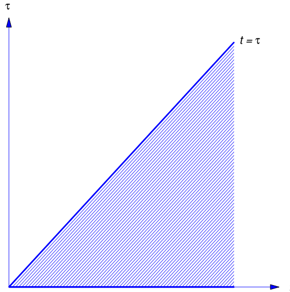
Figure 8.6.1 The region of integration for the convolution theorem
