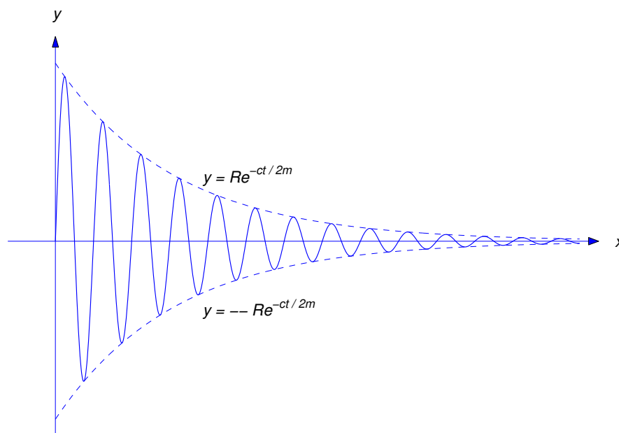
Figure 6.2.1 Underdamped motion
