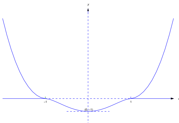
Figure 2.3.3 Two solutions of (2.3.12) on (-\infty, \infty) that coincide on (-1, 1) , but on no larger open interval
