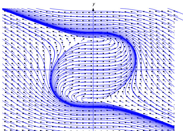
Figure 1.3.6 A direction field and integral curves for y' = \frac{x^2}{1 - x^2 - y^2}
