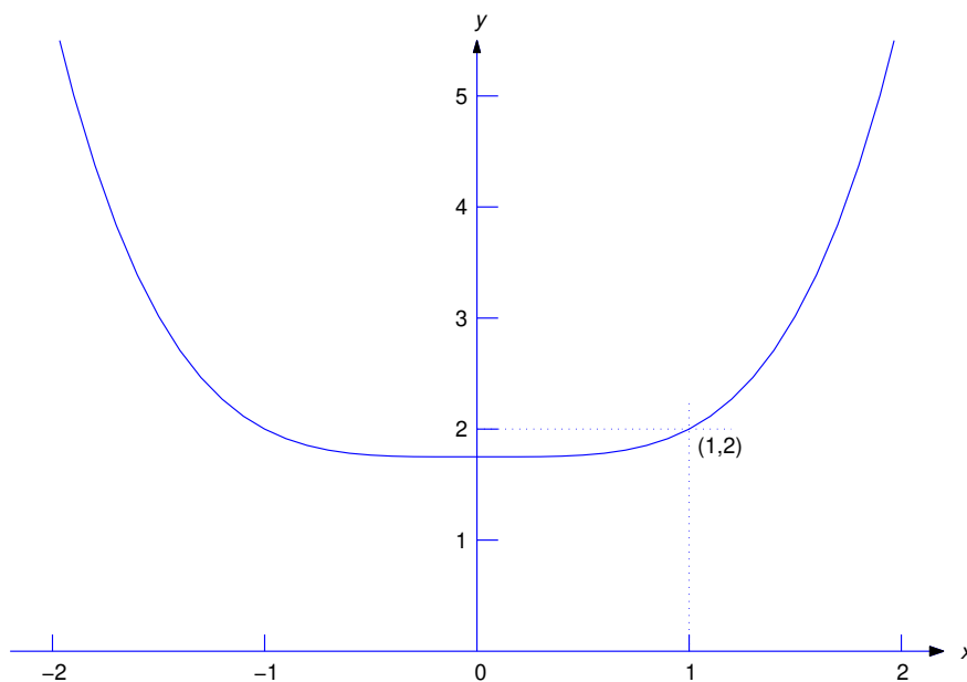
Figure 1.2.2 y = \frac{x^4 + 7}{4}
