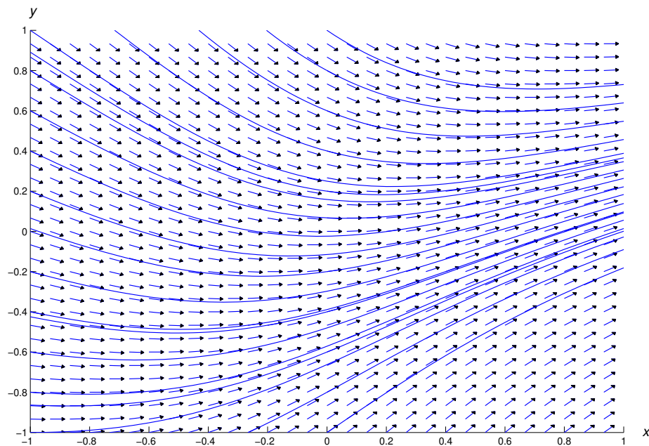
Figure 1.3.4 A direction field and integral curves for y' = \frac{x - y}{1 + x^2}
